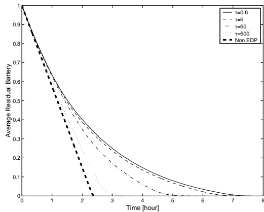
Fig. 3. Average remaining energy, without partition checking
