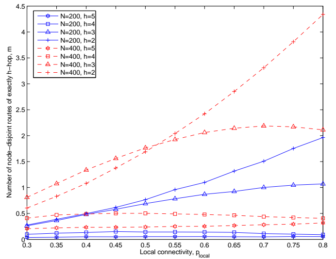
Fig. 5. Number of node-disjoint paths with exactly h -hops from source and destination.
